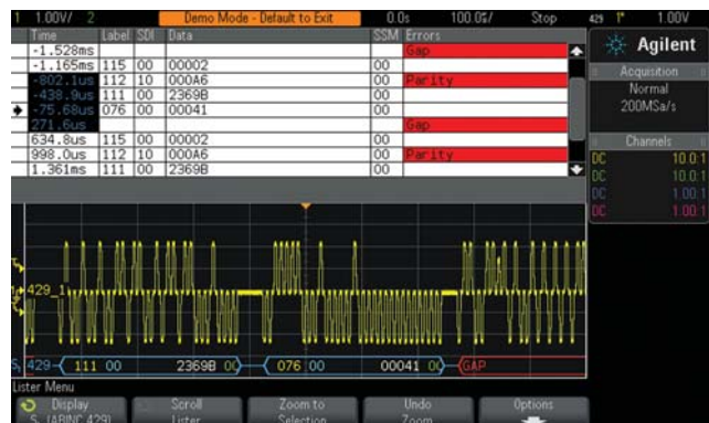
Figure 1: Decoding a differential ARINC 429 bus using an Agilent InfiniiVision 3000 X-Series oscilloscope reveals timing and parity errors.
